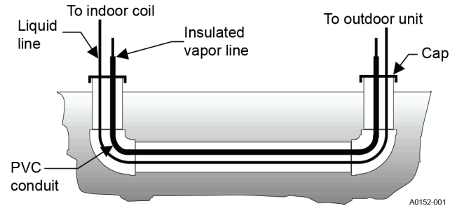
Figure 4: Underground installation
