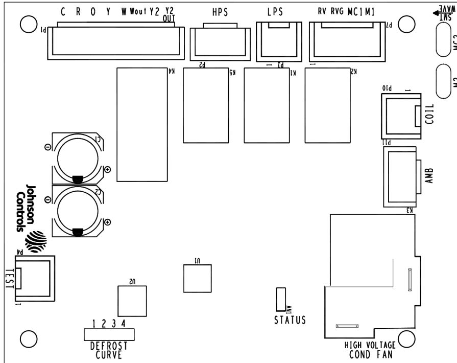
Figure 22: Demand defrost control module
