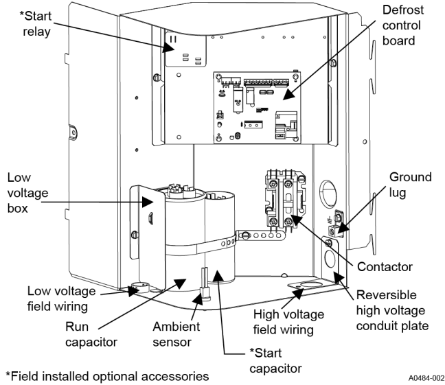
Figure 10: Outdoor unit control box (208/230 V single-phase 30, 36, 42, 48, and 60 models only)
