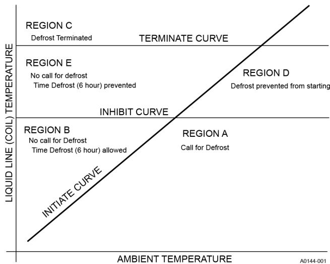
Figure 23: Defrost operation curves
