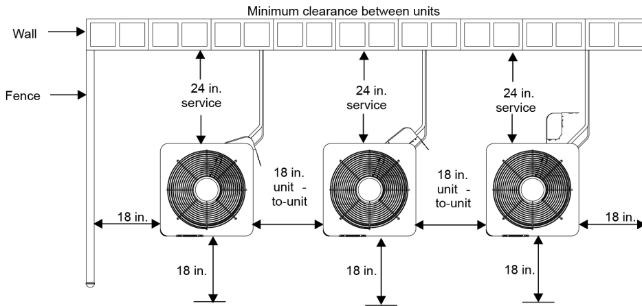
Figure 2: Alternative installation clearances
