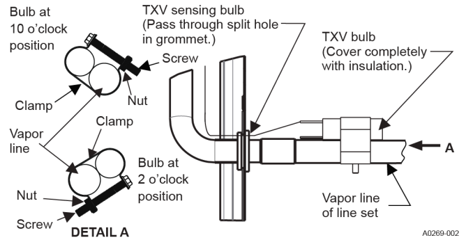
Figure 8: Proper bulb location
