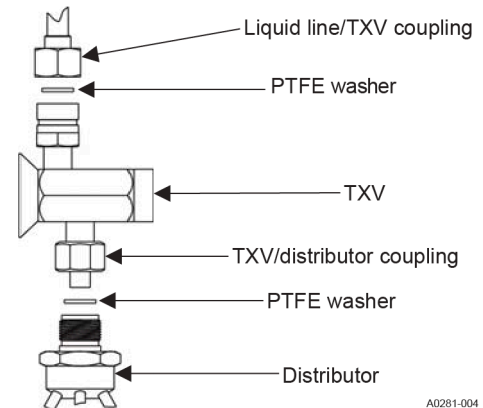
Figure 6: TXV installation
