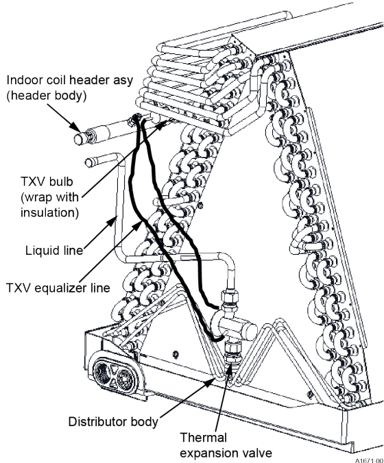
Figure 7: TXV bulb and equalizer line installations
