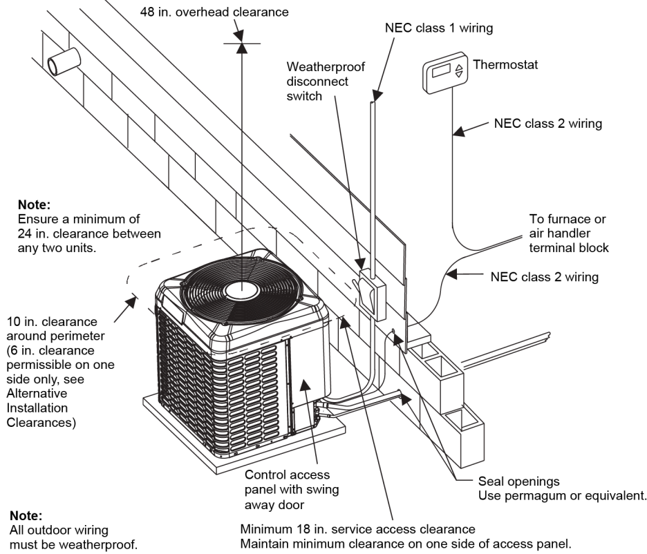
Figure 1: Typical installation clearances
