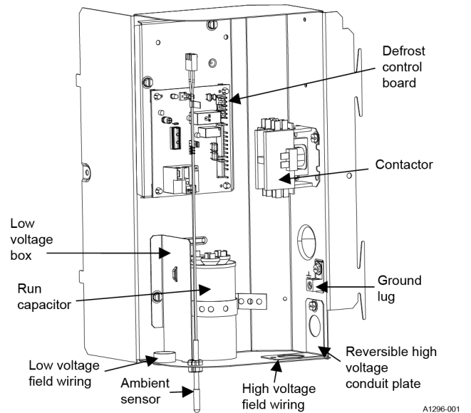
Figure 12: Outdoor unit control box (208/230 V single-phase 18 and 24 models only)
