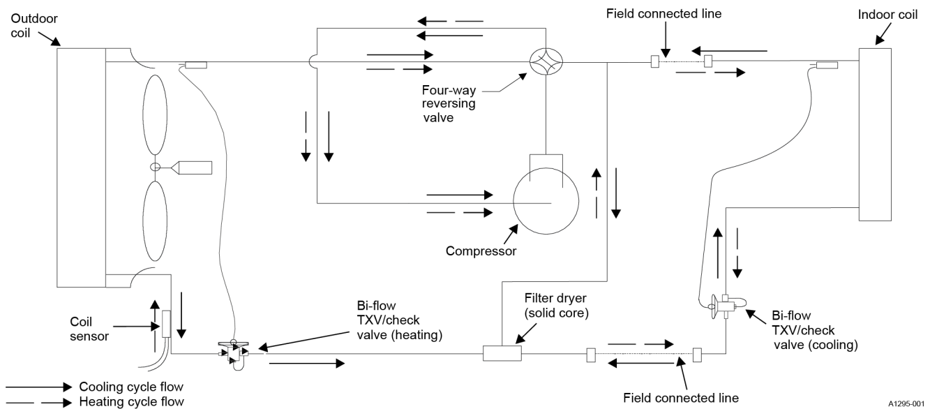
Figure 21: Heat pump flow diagram
